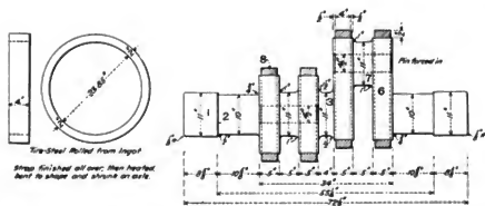
Figs. 1373-1376. Crank Axle for Four-Cylinder Balanced Compound Atlantic (4-4-2) Locomotive. C. B. & Q. Baldwin Locomotive Works.
